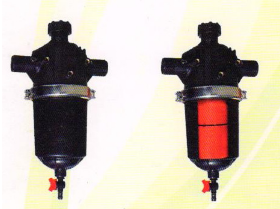
2" T Type Disc Filter (Industrial Plastic, 25m 3 /hr)
